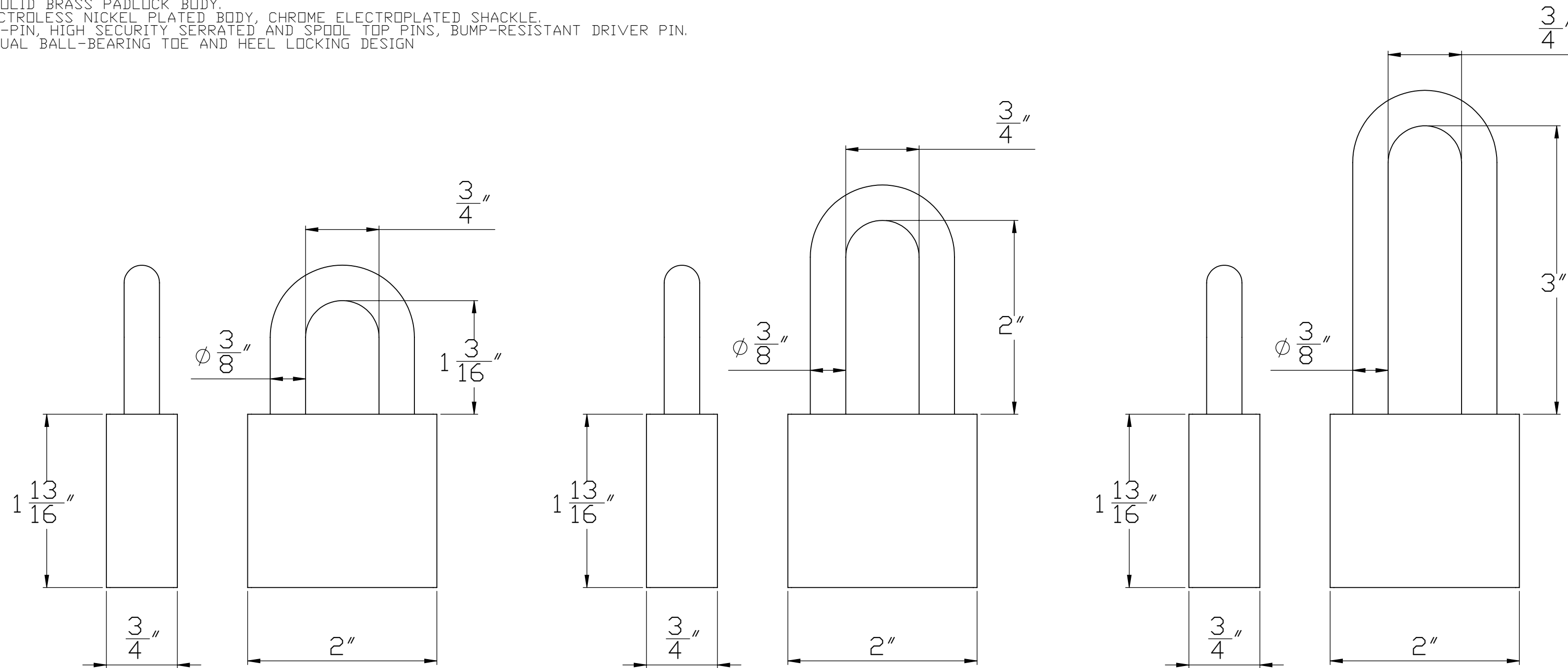
1" SHACKLE
