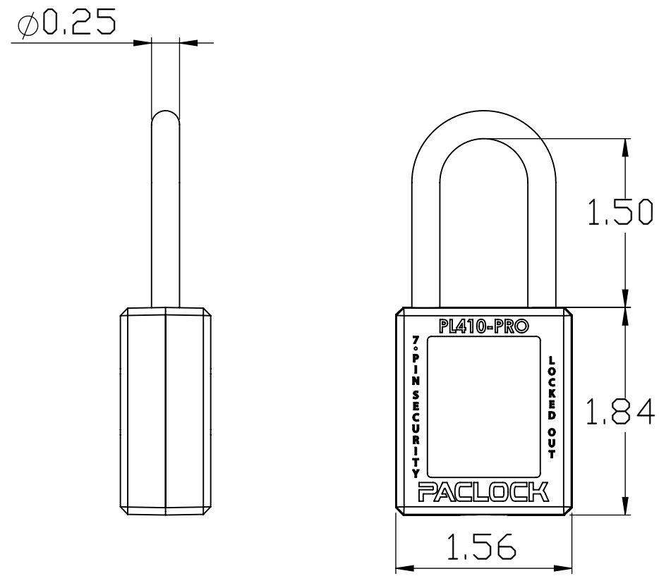
1-1/2" SHACKLE
